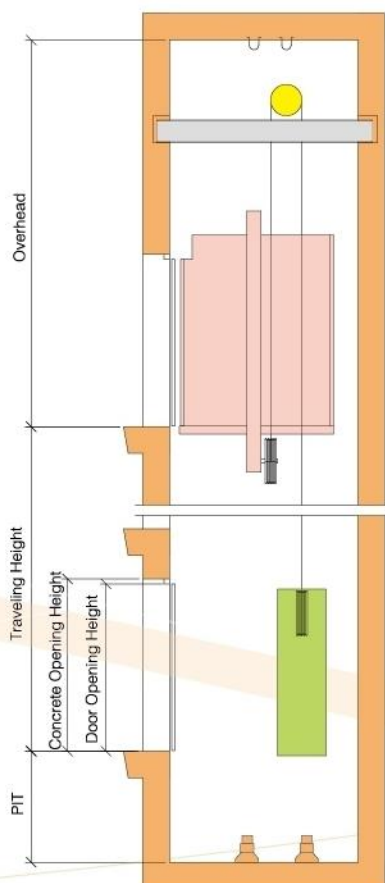
Hoistway Vertical Section View
