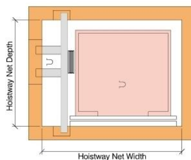
Hoistway Top Plan View
